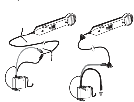
Figure 2a. Pair Tracing
