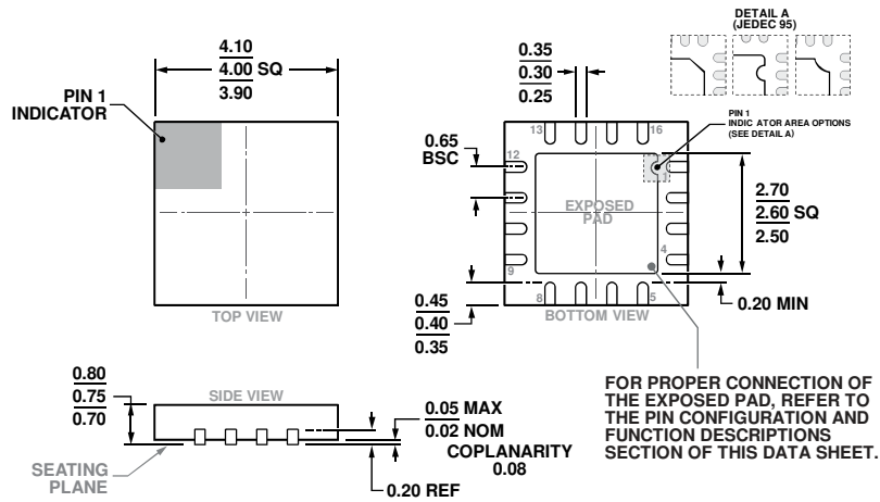
Figure 56. 16-Lead Lead Frame Chip Scale Package [LFCSOP] 4 mm × 4 mm Body, 0.75 mm Package Height (CP-16-17)
