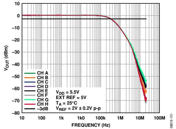
Figure 45. Multiplying Bandwidth
