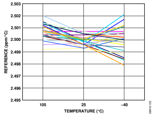
Figure 47. 2.5 V Reference Temperature Coefficient vs. Temperature
