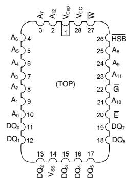
28-pin LCC
