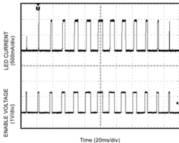
Enable (Frequency = 67Hz)
