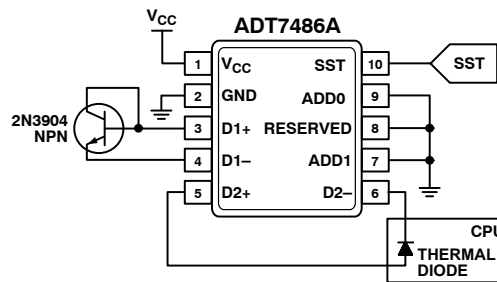
Figure 18. ADT7486A Typical Application Schematic
