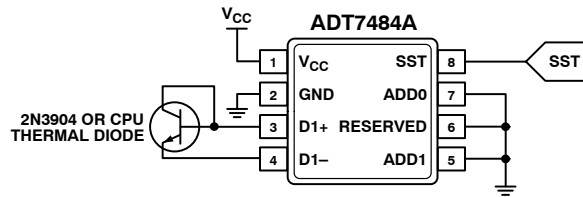
Figure 17. ADT7484A Typical Application Schematic
