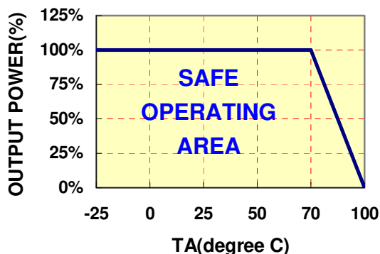
DERATING CURVES
