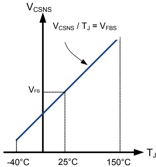
Figure 29. Temperature Reporting
