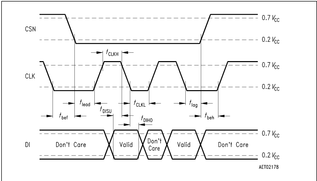
Figure 13 SPI-Input Timing
