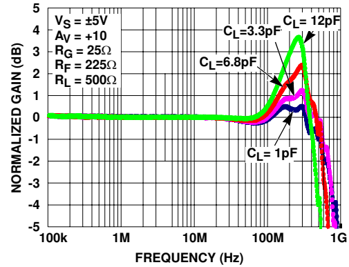
FIGURE 10. GAIN vs FREQUENCY FOR VARIOUS C_{LOAD} ( A_V = +10 )
