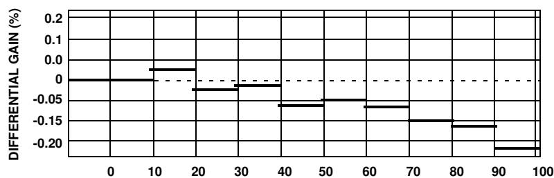
FIGURE 35. DIFFERENTIAL GAIN (%)
