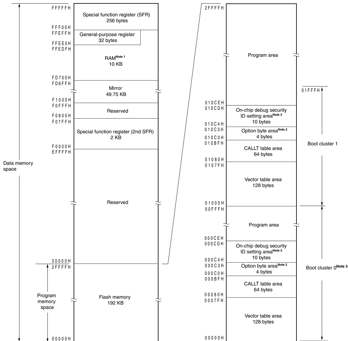
Figure 3-4. Memory Map ( \mu PD78F1155, 78F1155A)
