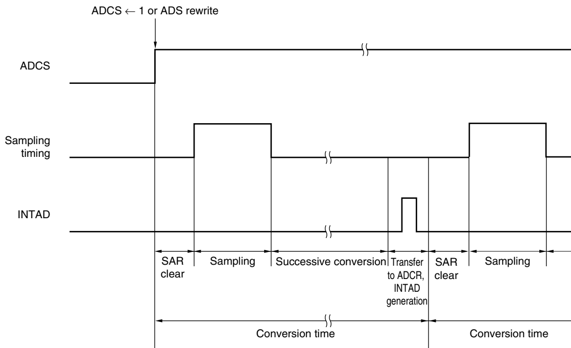
Figure 10-6. A/D Converter Sampling and A/D Conversion Timing
