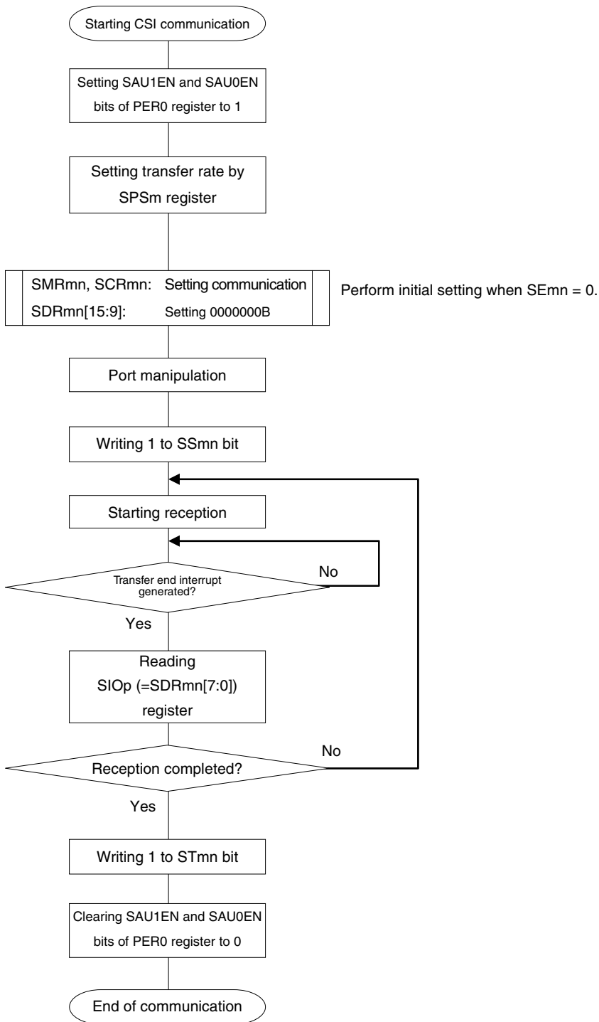
Figure 12-61. Flowchart of Slave Reception (in Single-Reception Mode)
