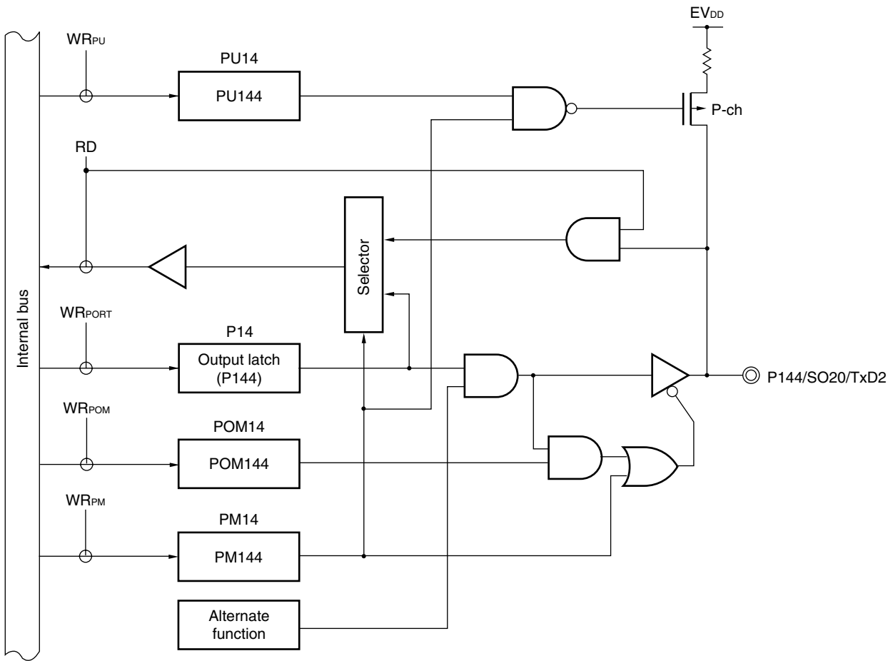
Figure 4-35. Block Diagram of P14
