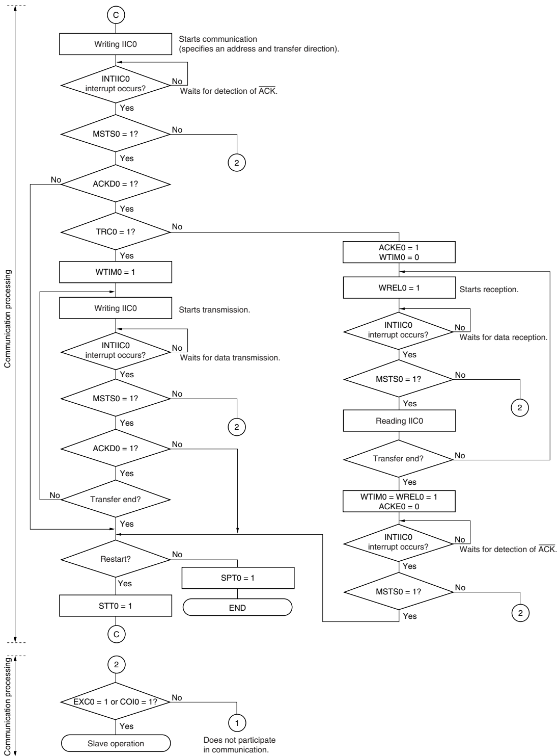
Figure 13-25. Master Operation in Multi-Master System (3/3)
