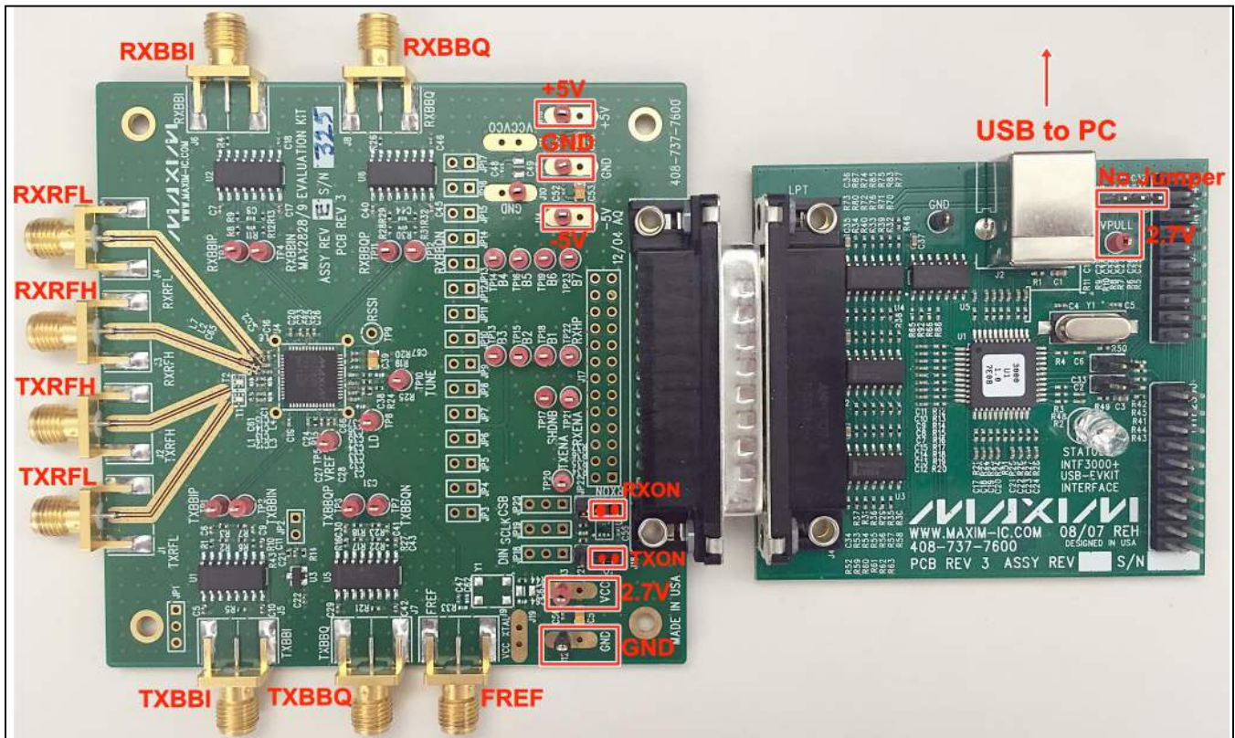
Figure 1. MAX2828/MAX2829 EV Kit Connections
