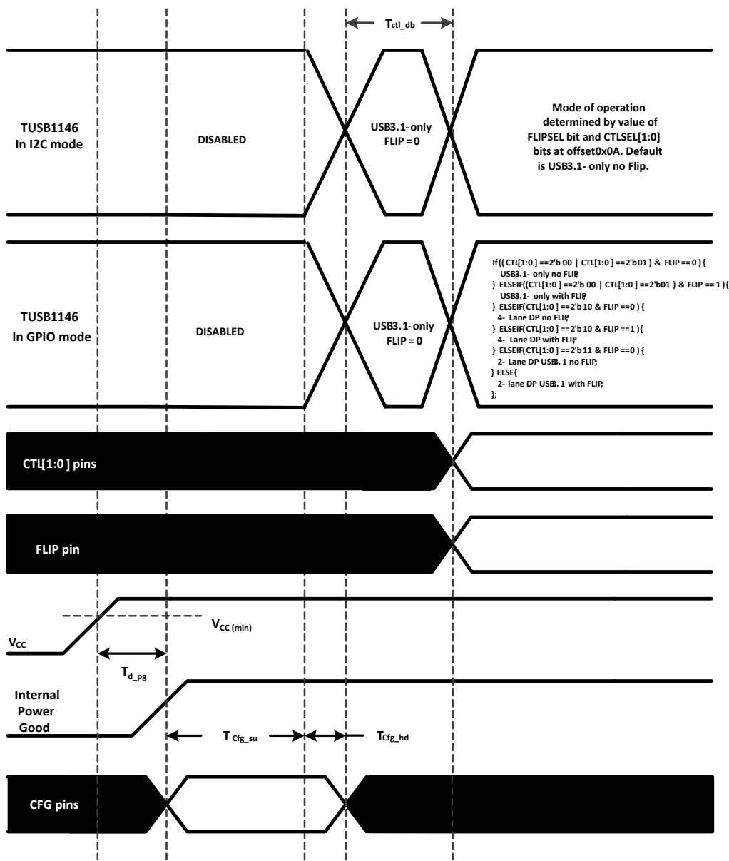
Figure 27. Power-On Timing
