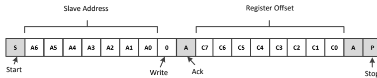
Figure 32. I2C Write without data
