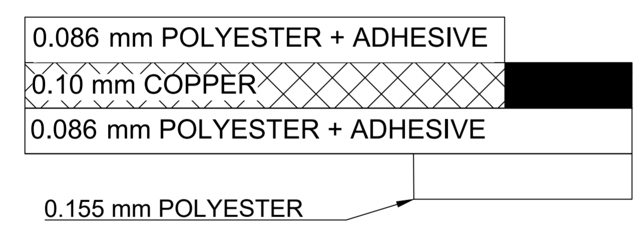
CROSS-SECTION
