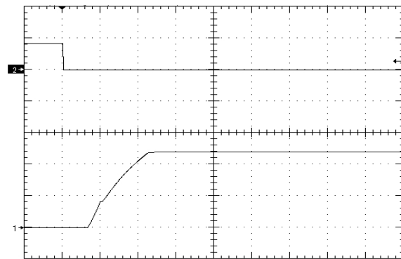
Figure 10. Startup Waveform via Enable Pin, time scale 10mS/div. Vin=Vin_nom, full resistive load + 820uF. Ch1=5V/div, Ch2=5V/div
