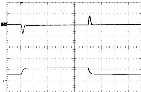
Figure 11. Load Transient Response (100mV/div), di/dt=0.1A/uS, 50% - 25% - 50% of full load, time scale: 200uS/div.
