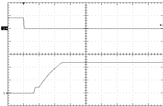
Figure 9. Startup Waveform via Enable Pin, time scale 10mS/div. Vin=Vin_nom, full load Ch1=5V/div, Ch2=5V/div
