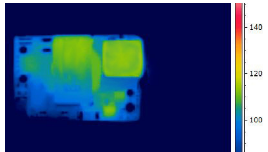
Figure 4. Thermal Image of CPT3B48 (2.5A output, 85C Ambient, natural convection, Vin = 48V, airflow from pin 3 to pin 1, T max = 111 °C)
