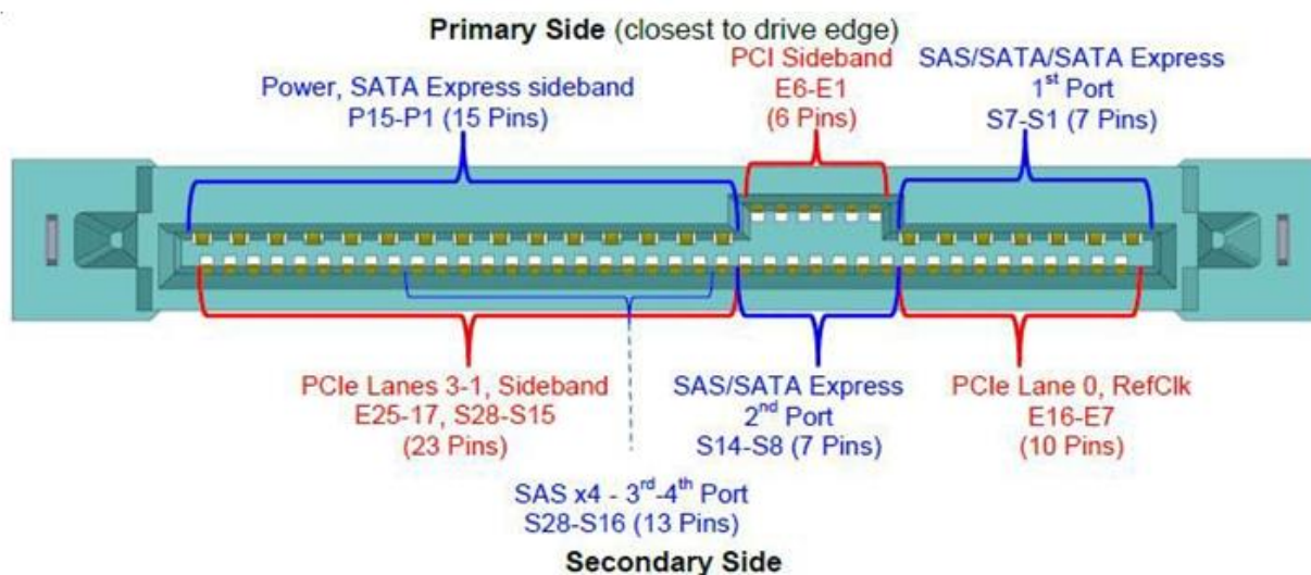
Figure 5-1 EMP I PRO U.2 PCIe SSD Pin Locations
