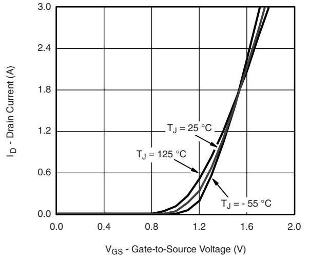
T_J = 25\text{ °C} T_J = 125\text{ °C} T_J = -55\text{ °C} Transfer Characteristics
