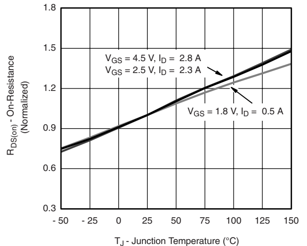
V_{GS} = 4.5\text{ V}, I_D = 2.8\text{ A} V_{GS} = 2.5\text{ V}, I_D = 2.3\text{ A} V_{GS} = 1.8\text{ V}, I_D = 0.5\text{ A} On-Resistance vs. Junction Temperature
