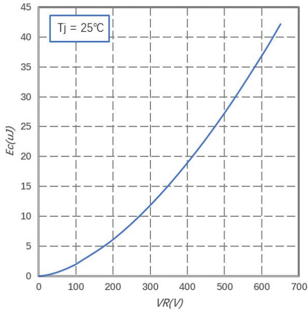
Fig.5-Capacitance Stored Energy
