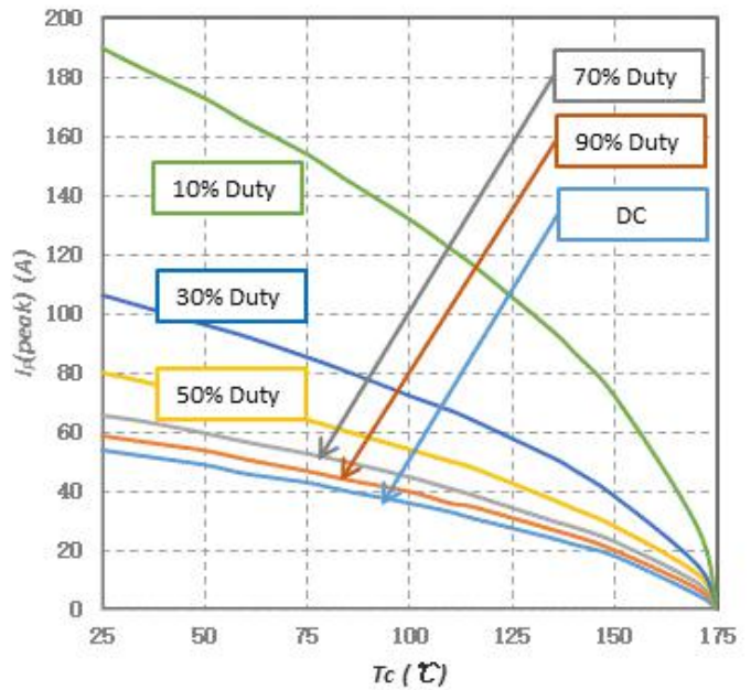
Fig.8-Current Derating
