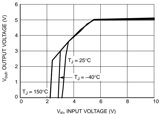
Figure 5. Output Voltage vs. Input Voltage ( R_{LOAD} = 51\text{ k} , I_{out} = 100\ \mu\text{A} )
