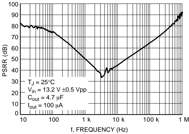
Figure 14. Ripple Rejection vs. Frequency
