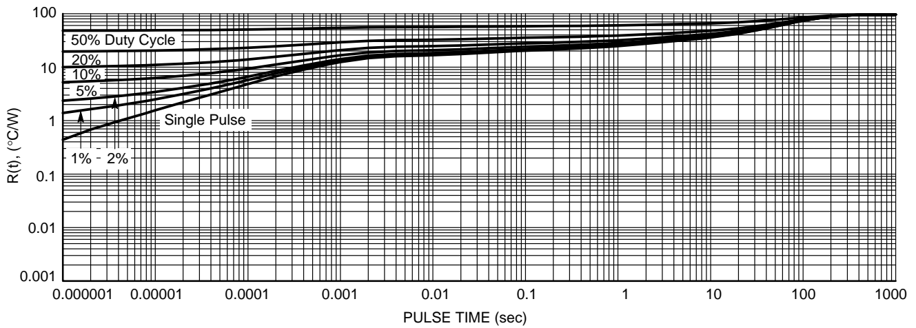
Figure 21. Transient Thermal Response (SOIC-8 Fused) Cu Area = 645 mm 2
