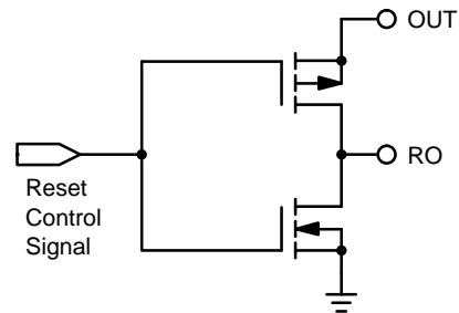
Figure 18. Reset Output Circuitry
