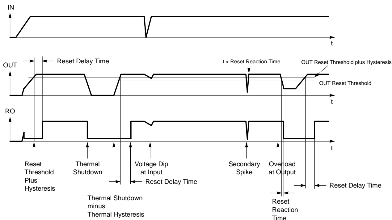
Figure 19. Reset Timing
