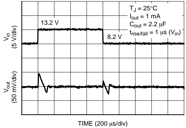
Figure 13. Line Transient
