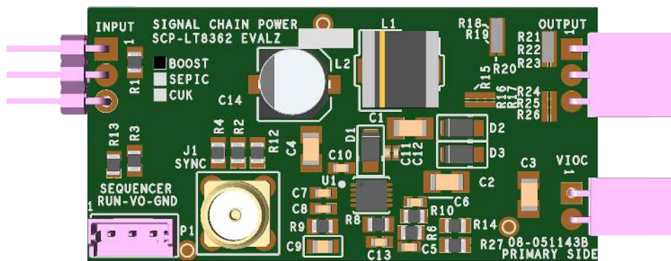
Figure 1. SCP-LT8362-B-EVALZ Board
