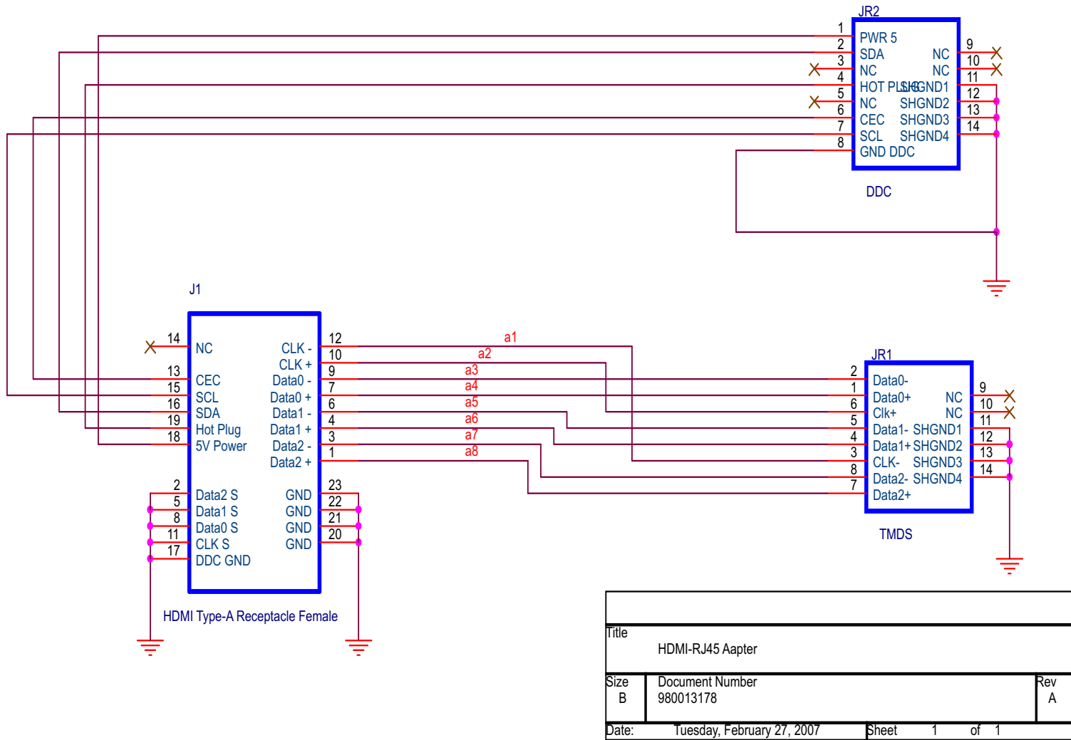
Figure 2. Schematic (Passive Adapter Board)
