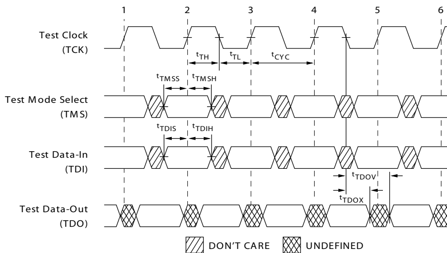
Figure 2. TAP Timing
