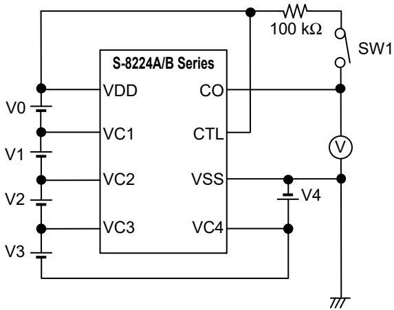
Figure 5 Test Circuit 1
