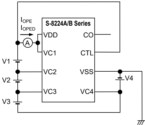
Figure 7 Test Circuit 3
