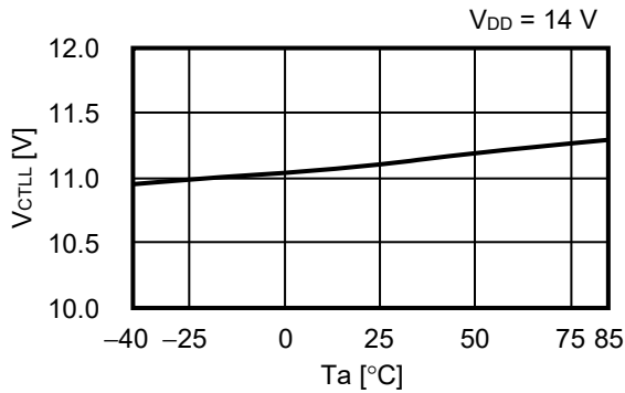
4.1 V_{CTL} vs. T_a
