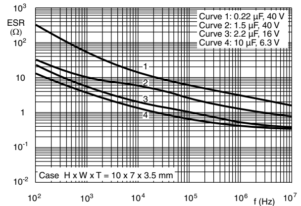
Fig. 13 - Typical ESR at 25^\circ\text{C} as a function of frequency
