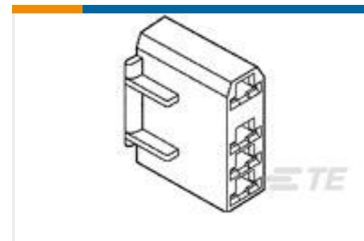
TE Part #520987-2 250 FASTON HSG. REC 4P NATURAL
