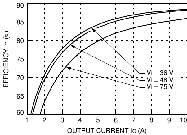
Figure 4. Typical QHW050A1-Q Converter Efficiency vs. Output Current at Room Temperature
