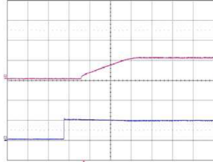
Start-up enabled by connecting V_i at: T_{ref} = +25^{\circ}C , V_i = 5 V , I_o = 30 A resistive load. Top trace: output voltage (1 V/div.). Bottom trace: input voltage (5 V/div.). Time scale: (5 ms/div.).
