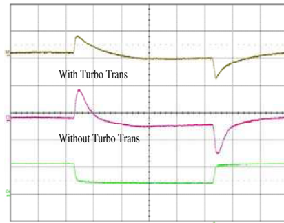
Output voltage response to load current step-change (7.5-22.5-7.5 A) at: T_{ref} = +25^{\circ}C , V_i = 5 V . Top trace: output voltage (100 mV/div.). Middle trace: output voltage (100mV/div.). Bottom trace: load current (20 A/div.). Time scale: (0.1 ms/div.).
