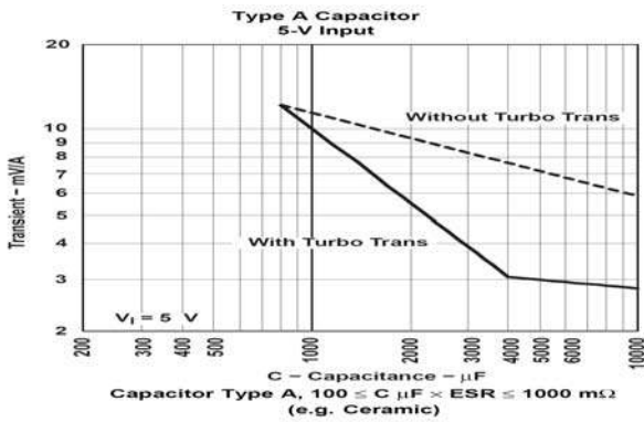
Type A TurboTrans C 0 Values & Required R TT Selection Table
