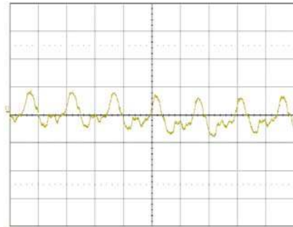
Output voltage ripple at: T_{ref} = +25^{\circ}C , V_i = 5 V , I_o = 30 A resistive load. Trace: output voltage (2 mV/div.). Time scale: (2 \mu s/div.).
