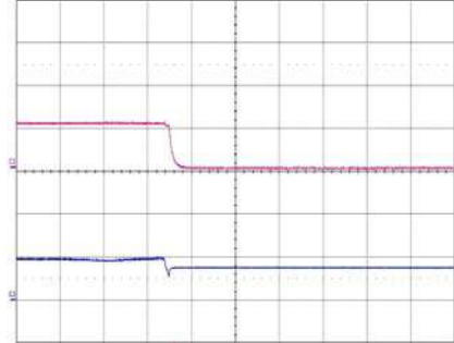
Shut-down enabled by disconnecting V_i at: T_{ref} = +25^{\circ}C , V_i = 5 V , I_o = 30 A resistive load. Top trace: output voltage (1 V/div.). Bottom trace: input voltage (5 V/div.). Time scale: (0.5 ms/div.).
