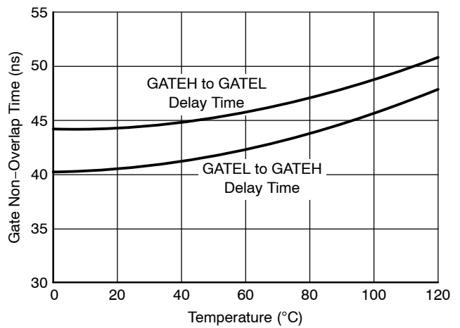
Figure 14. GATE Non-Overlap Times vs. Temperature
