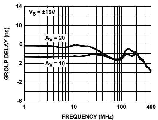
FIGURE 28. GROUP DELAY
