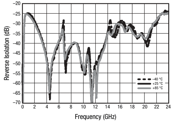
Figure 10. Small Signal Reverse Isolation (IS12) vs Frequency and Temperature, Wide Band
