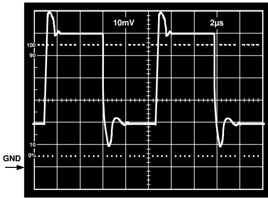
Figure 38. V_S = 5\text{ V}, 0\text{ V} ; Unity-Gain Follower Response to 40 mV Step, Centered 40 mV above Ground, R_L = 10\text{ k}\Omega
