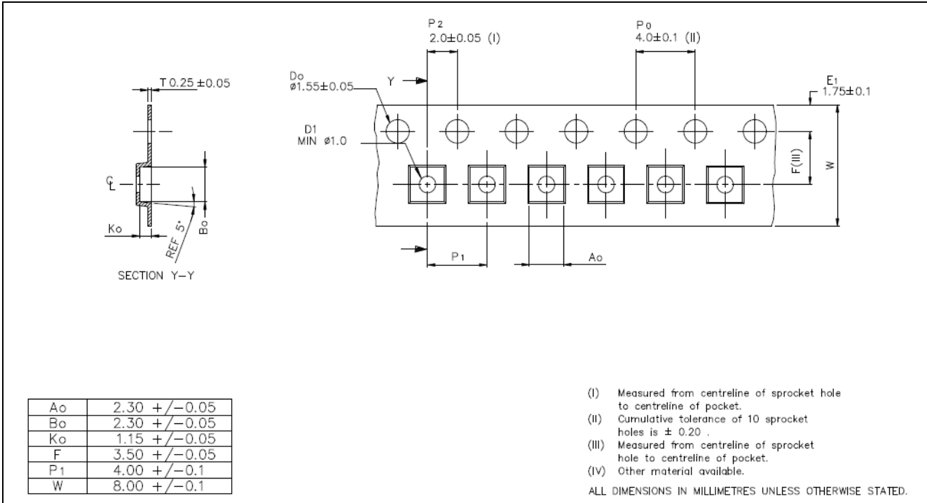
Figure 17. Carrier tape
