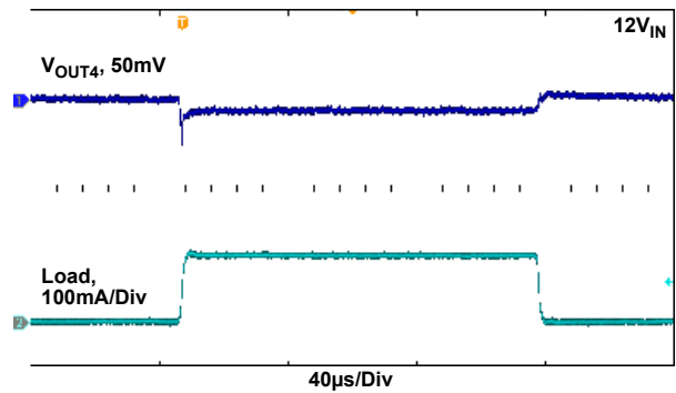
Figure 25. V_{OUT4} Load Transient, 0A/0.15A
