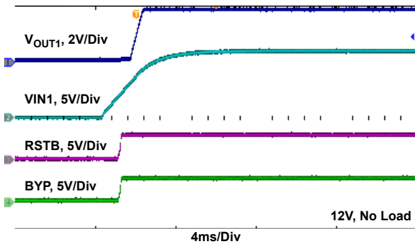
Figure 34. Startup with VIN1 Ramp: V OUT1 , VIN1, RSTB, BYP
