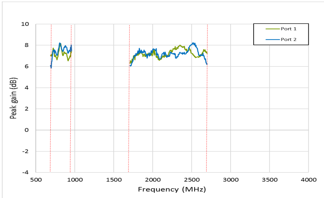
Figure 7. Peak gain (dBi)
