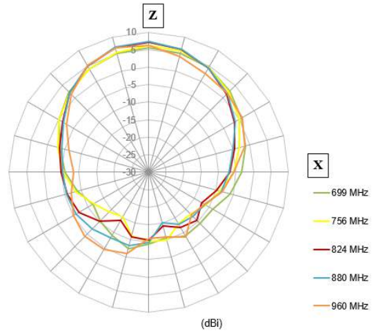
Figure 16. Z-X polar plots on target
