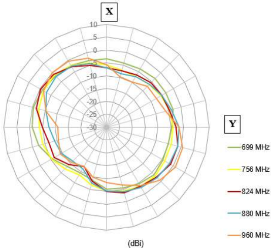
Figure 15. X-Y polar plots on target bands
