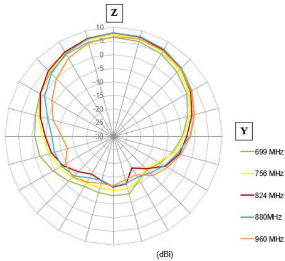
Figure 17. Z-Y polar plot on target bands
