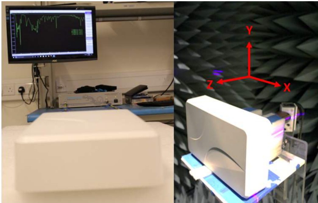
Figure 2. VNA test setup (left) and anechoic chamber test setup (right)
