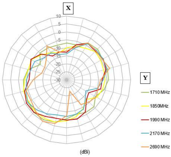
Figure 12. X-Y polar plots on target bands
