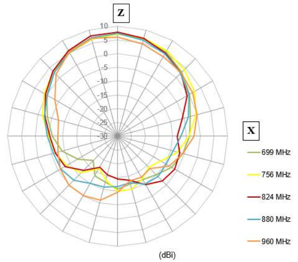
Figure 10. Z-X polar plot on target bands
