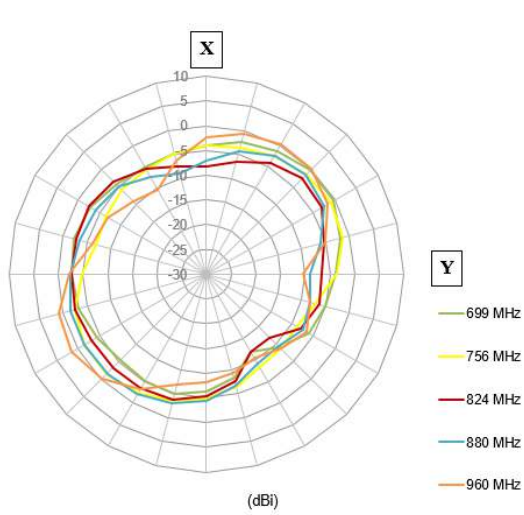
Figure 9. X-Y polar plot on target bands
