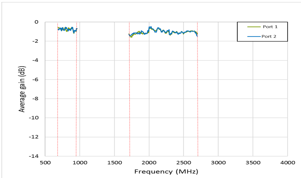
Figure 8. Average gain (dB)
