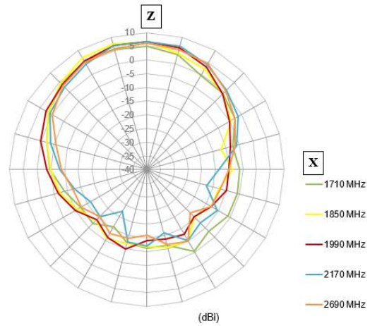
Figure 19. Z-X polar plot on target bands
