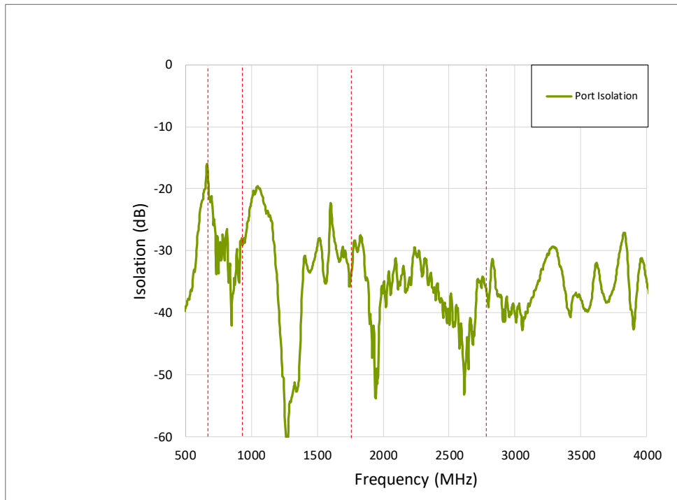
Figure 4. Isolation (dB) S21
