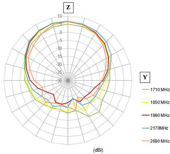
Figure 14. Z-Y polar plots on target bands
