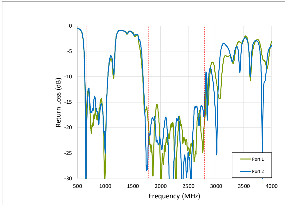
Figure 3. Return Loss (dB) S11
