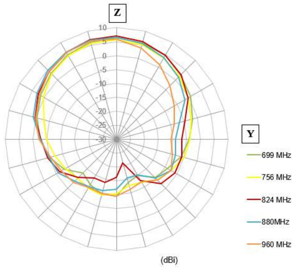
Figure 11. Z-Y polar plot on target bands
