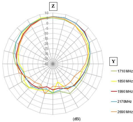
Figure 20. Z-Y polar plot on target bands
