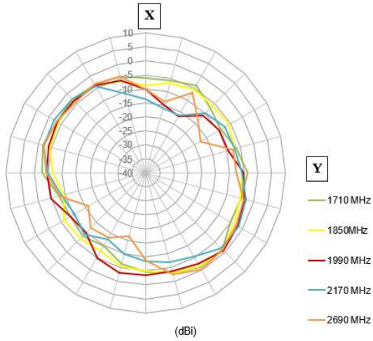
Figure 18. X-Y polar plot on target bands
