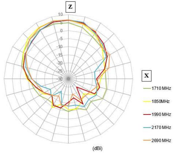
Figure 13. Z-X polar plots on target bands
