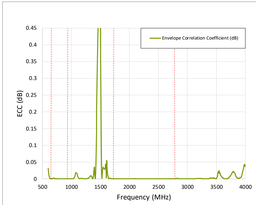
Figure 5. Envelope Correlation Coefficient (ECC)
