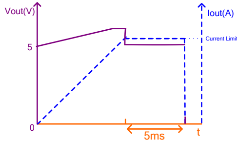
Figure 7: Over-Current Limit
