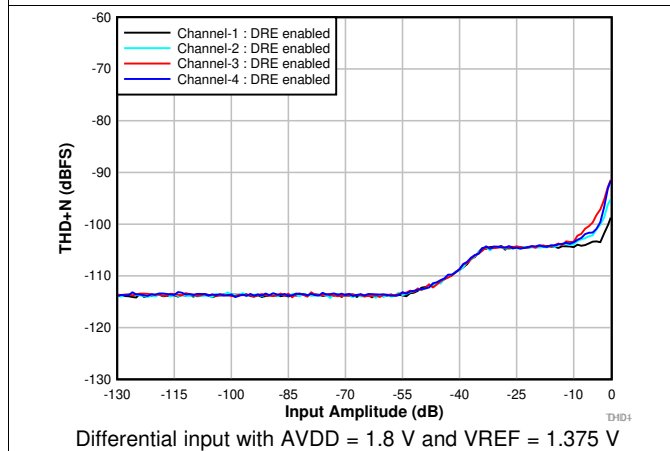
Figure 9. THD+N vs Input Amplitude With DRE Enabled
