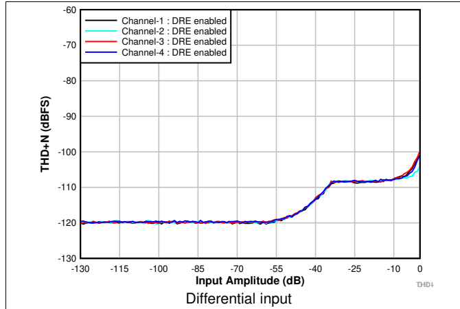
Figure 5. THD+N vs Input Amplitude With DRE Enabled
