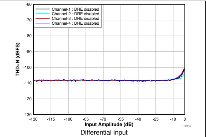
Figure 6. THD+N vs Input Amplitude With DRE Disabled
