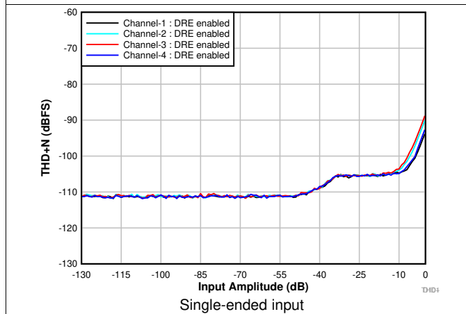
Figure 7. THD+N vs Input Amplitude With DRE Enabled
