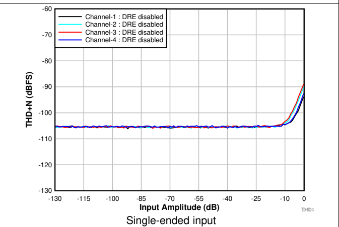
Figure 8. THD+N vs Input Amplitude With DRE Disabled
