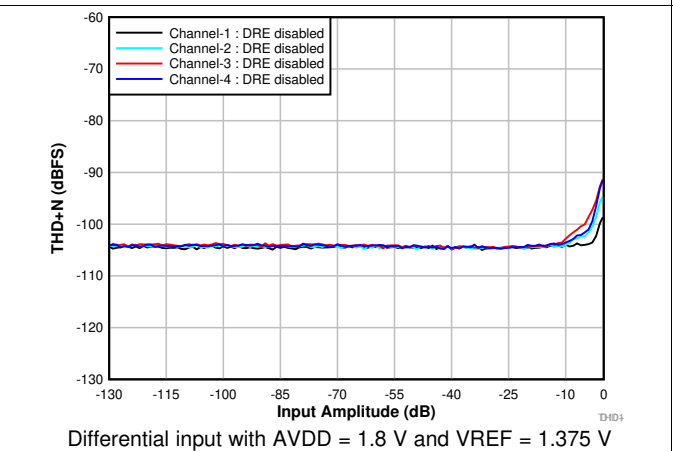
Figure 10. THD+N vs Input Amplitude With DRE Disabled
