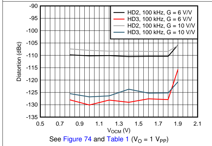
Figure 35. Noninverting Harmonic Distortion vs Output Common-Mode Voltage
