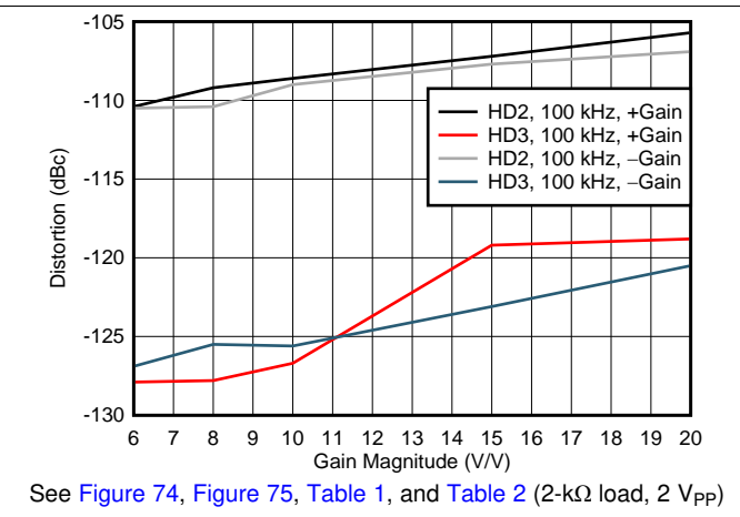
Figure 34. Harmonic Distortion vs Gain
