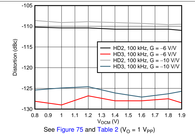
Figure 36. Inverting Harmonic Distortion vs Output Common-Mode Voltage
