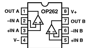
8-Lead Plastic DIP (P Suffix)
