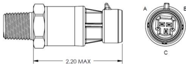
PACKARD CONNECTOR
