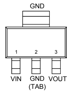
RT9074-25/33/50 SOT-223
