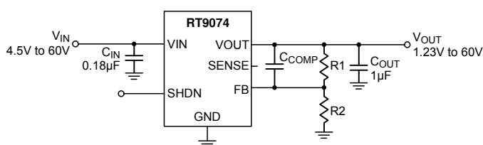
Figure 2. RT9074 Adjustable Output Above 25V
