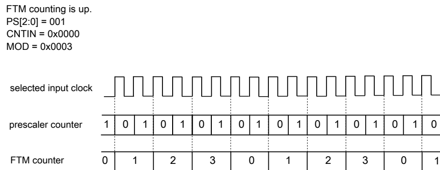
Figure 12-7. Example of the prescaler counter
