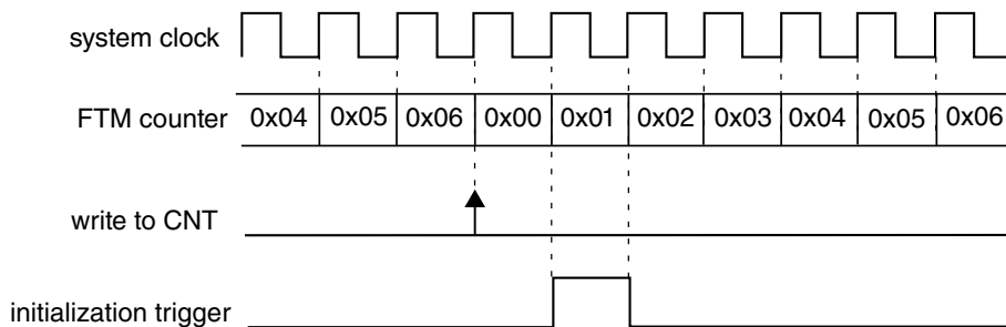
Figure 12-78. Initialization trigger is generated when there is a write to CNT register
