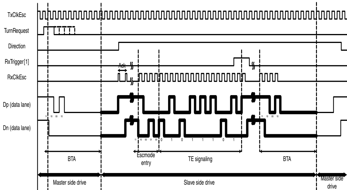
Figure 13-45. TE Signaling
