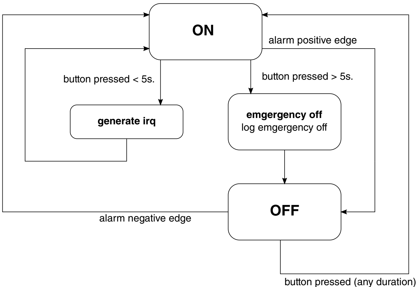
Figure 6-8. FSM
