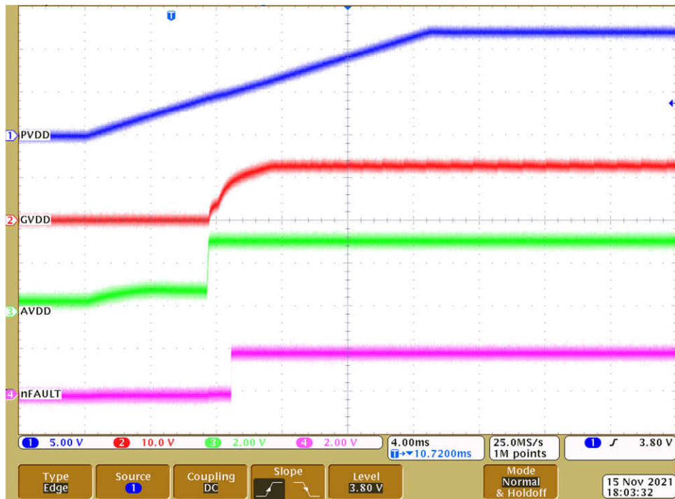
Figure 9-12. AVDD powerup
