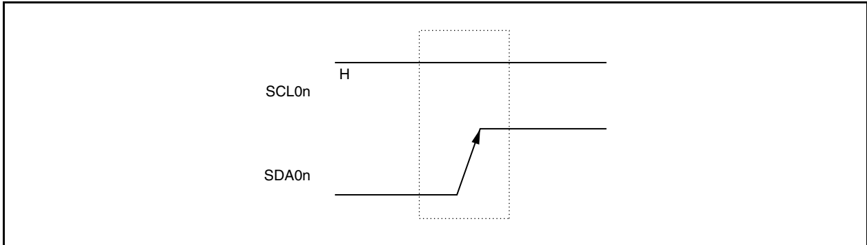
Figure 17-12. Stop Condition
