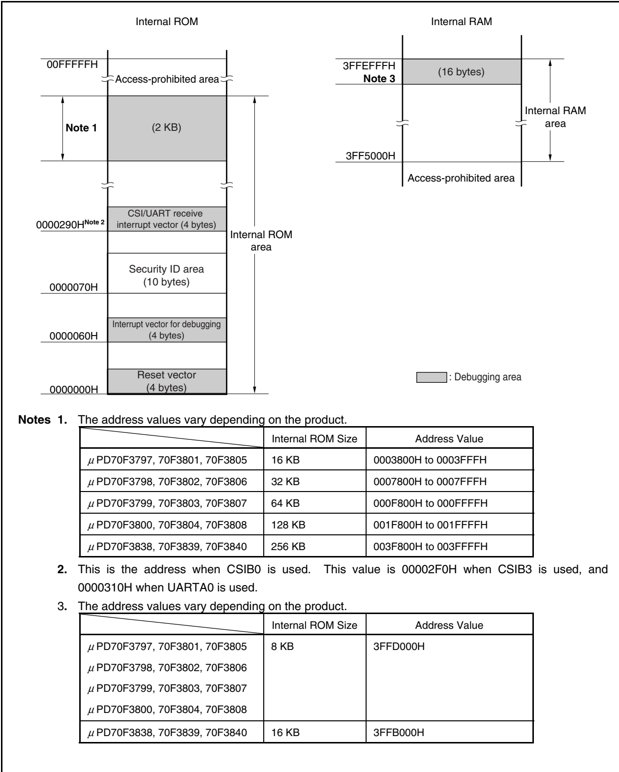
Figure 29-5. Memory Spaces Where Debug Monitor Programs Are Allocated
