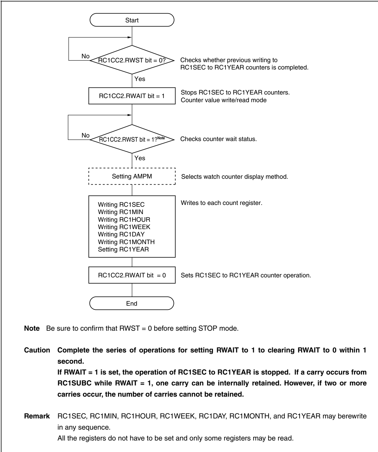
Figure 10-3. Rewriting Each Counter During Clock Operation
