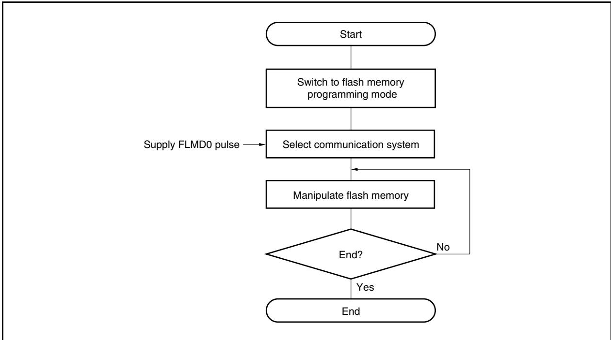
Figure 28-6. Procedure for Manipulating Flash Memory
