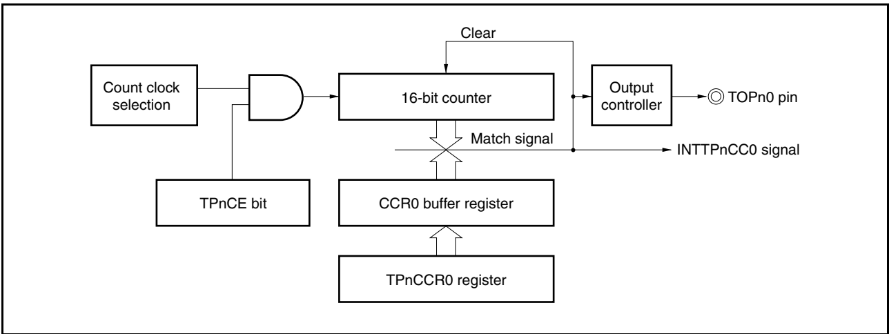
Figure 6-6. Configuration of Interval Timer
