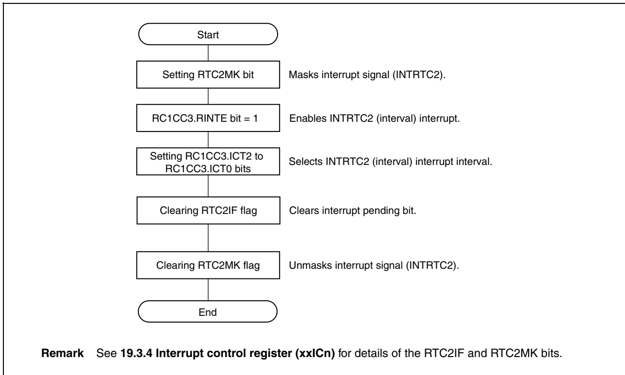
Figure 10-8. Changing INTRTC2 Interrupt Setting During Clock Operation
