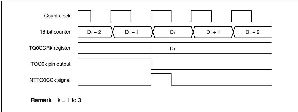
Figure 7-37. Timing of Generating Compare Match Interrupt Signal (INTTQ0CCk)
