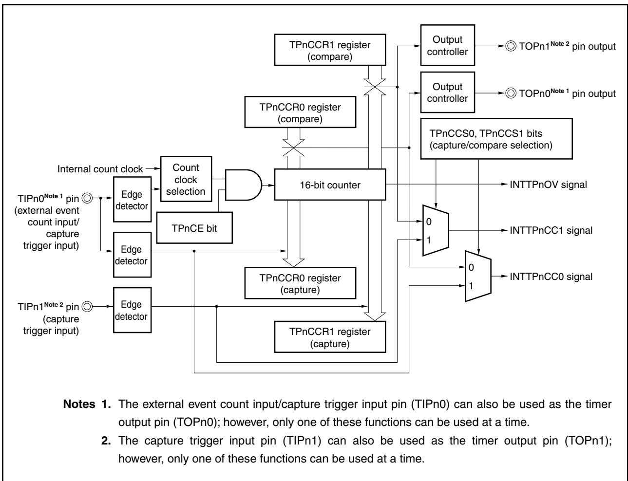
Figure 6-52. Configuration of TMPn in Free-Running Timer Mode
