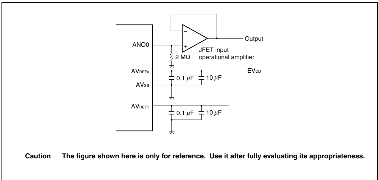
Figure 14-2. Example of External Pin Connection
