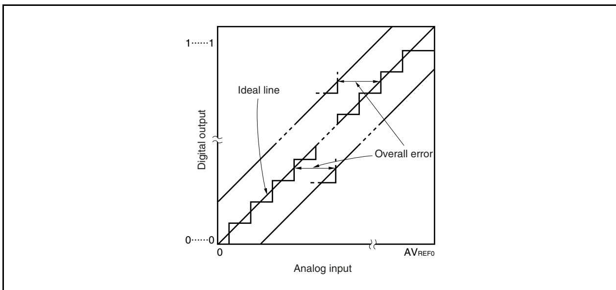
Figure 13-16. Overall Error
