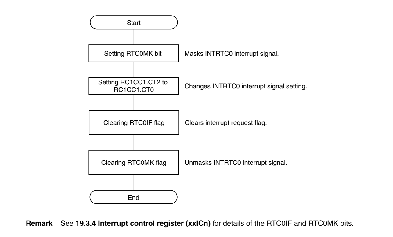
Figure 10-5. Changing INTRTC0 Interrupt Setting During Clock Operation
