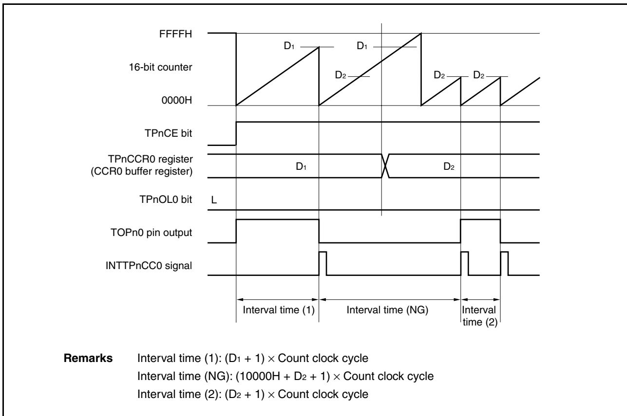
Figure 6-12. Rewriting TPnCCR0 Register
