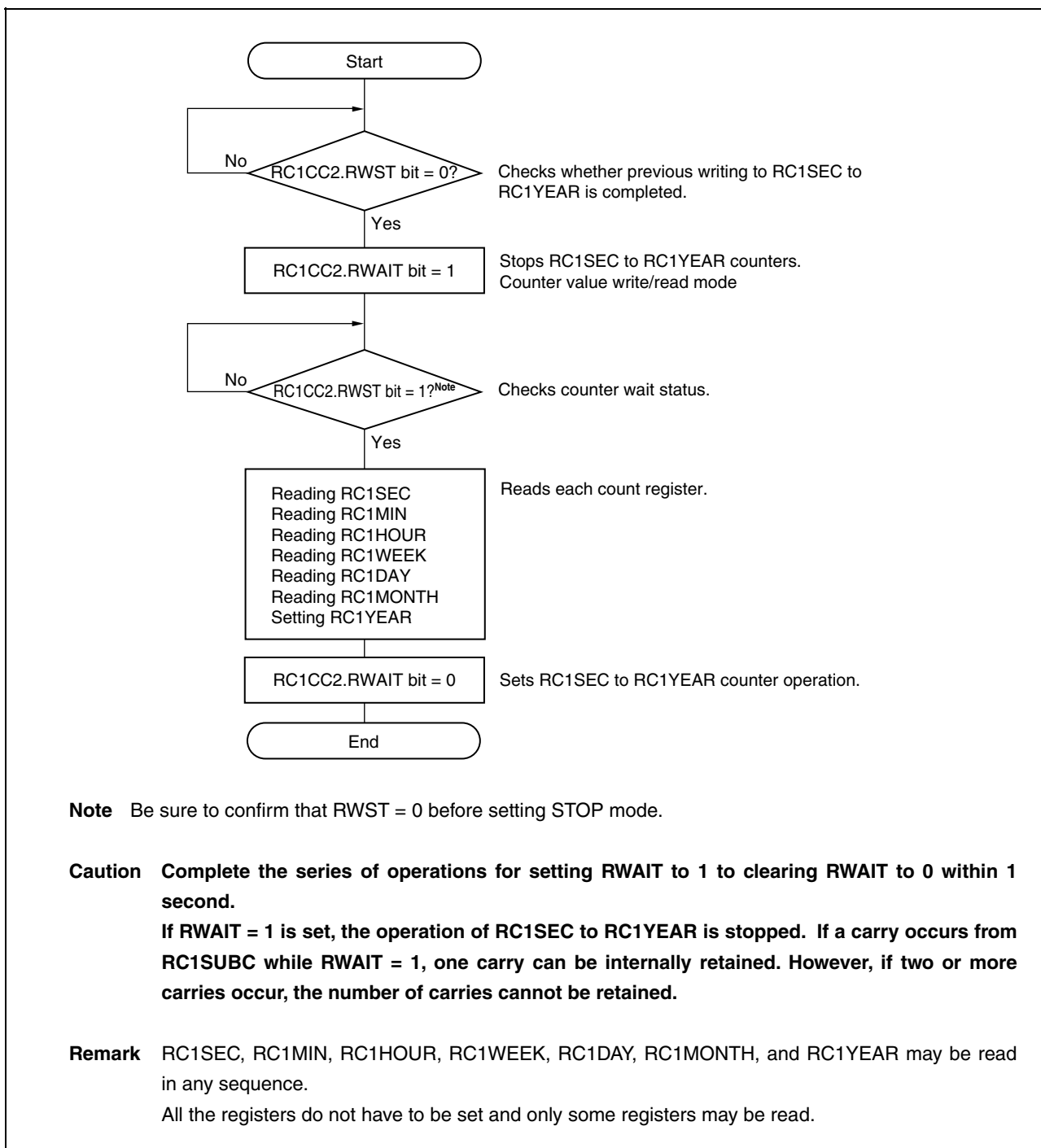
Figure 10-4. Reading Each Counter During Clock Operation
