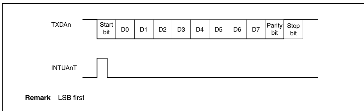
Figure 15-6. UART Transmission
