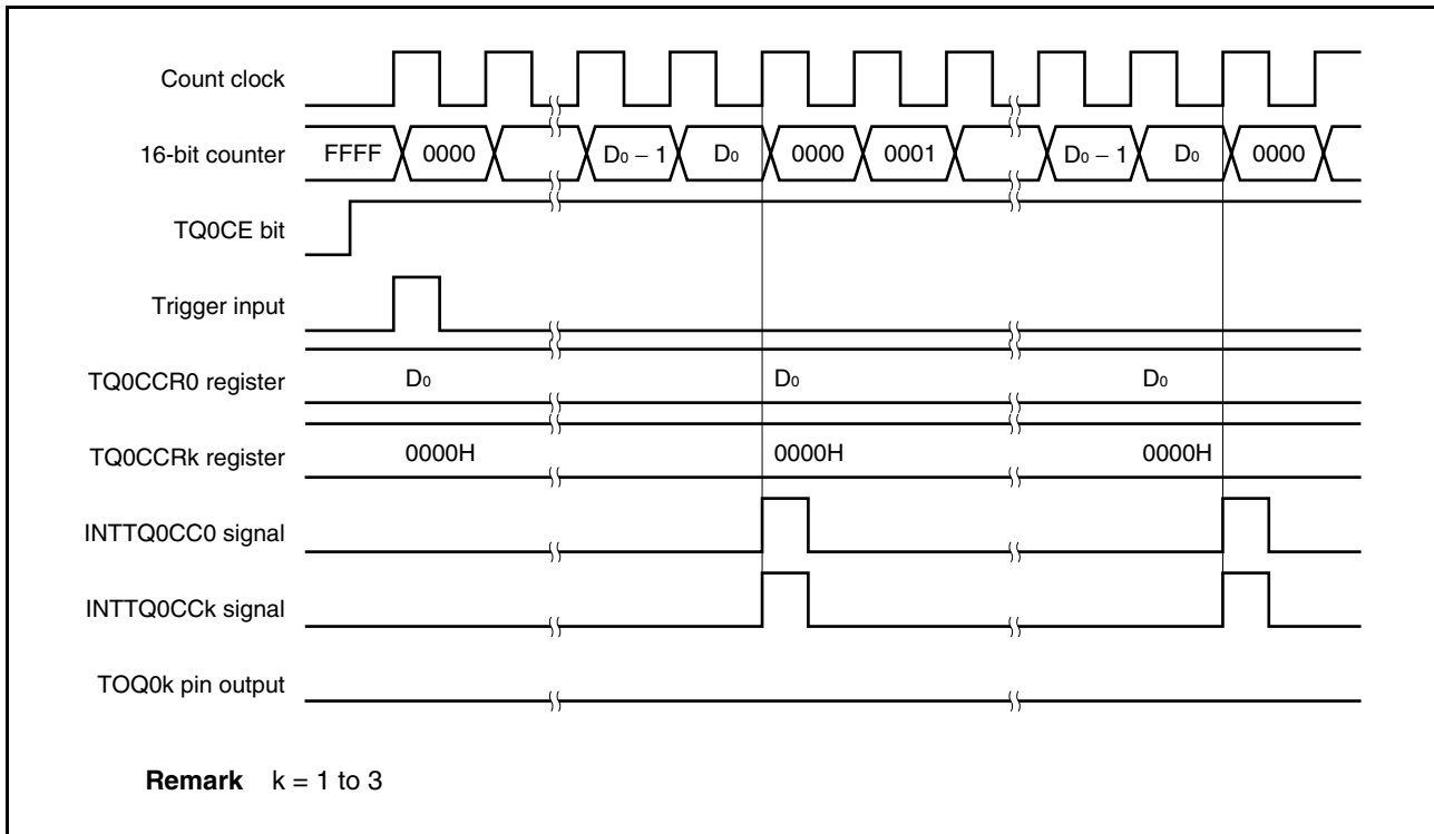
Figure 7-31. Outputting 0% PWM Waveform
