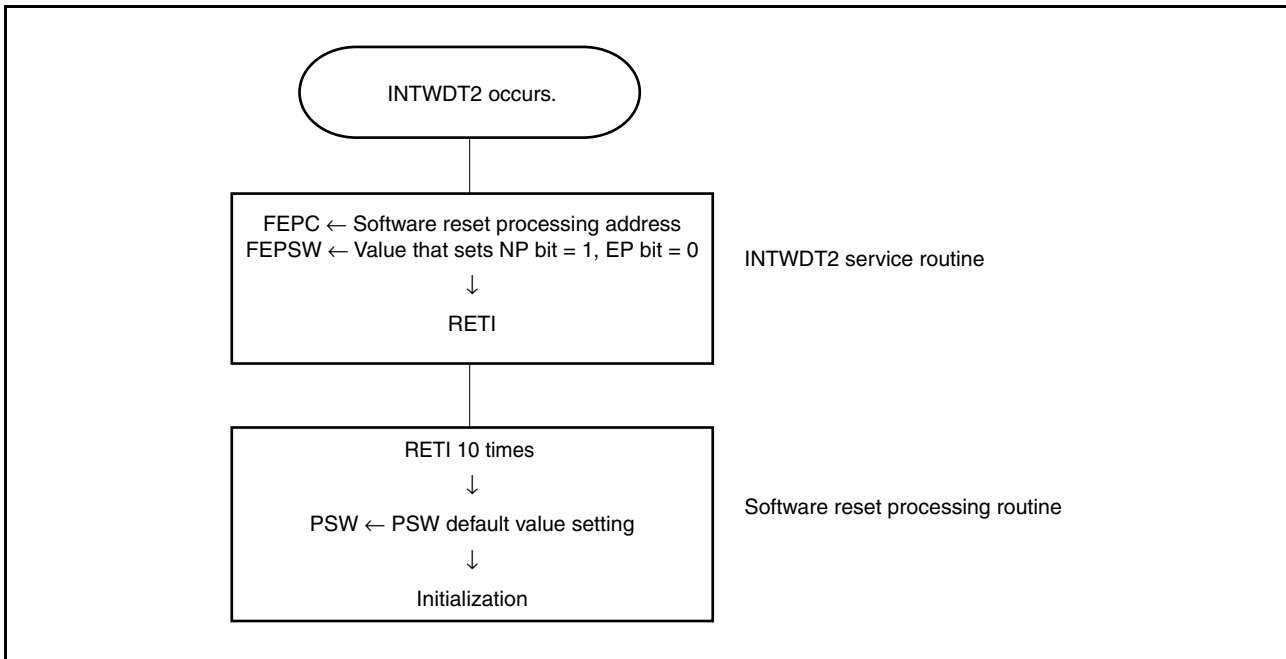
Figure 19-4. Software Reset Processing
