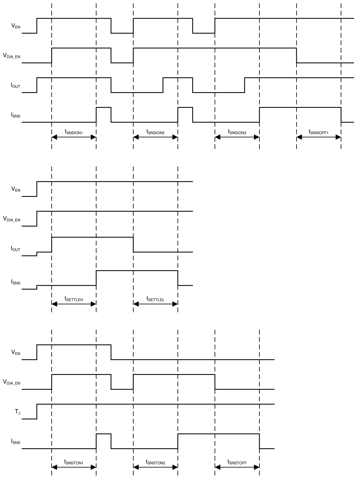
Figure 31. SNS Timing Characteristics Definitions
