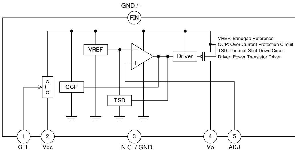
Figure 3. Block Diagram
