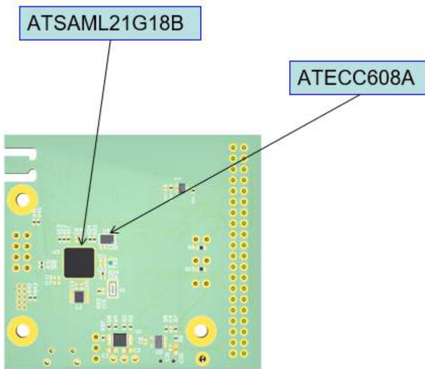
Figure 1-3. Bottom Side
