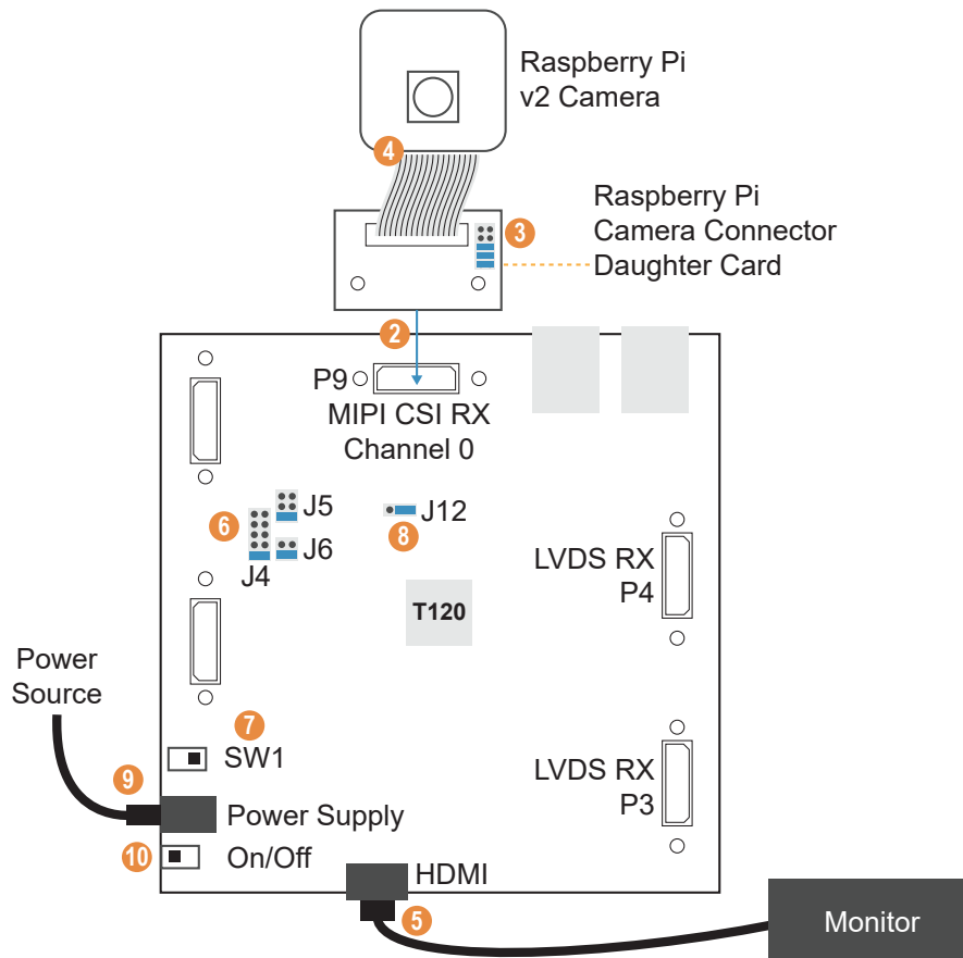
Figure 11: Hardware Setup
