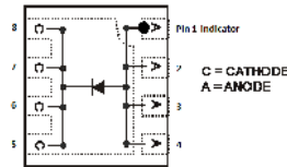
Top View Schematic and Pin Configuration
