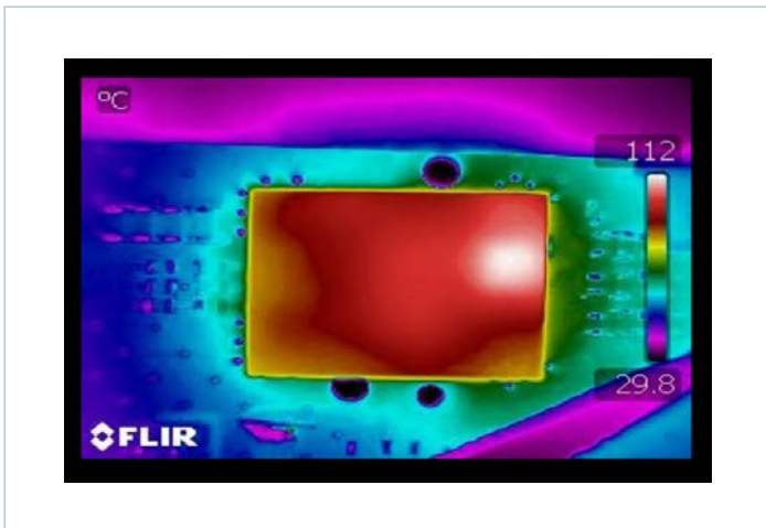
Figure 30 — Thermal image ( V_{IN} = 52V , I_{OUT} = 3.3A , CR, OLFM evaluation PCB)
