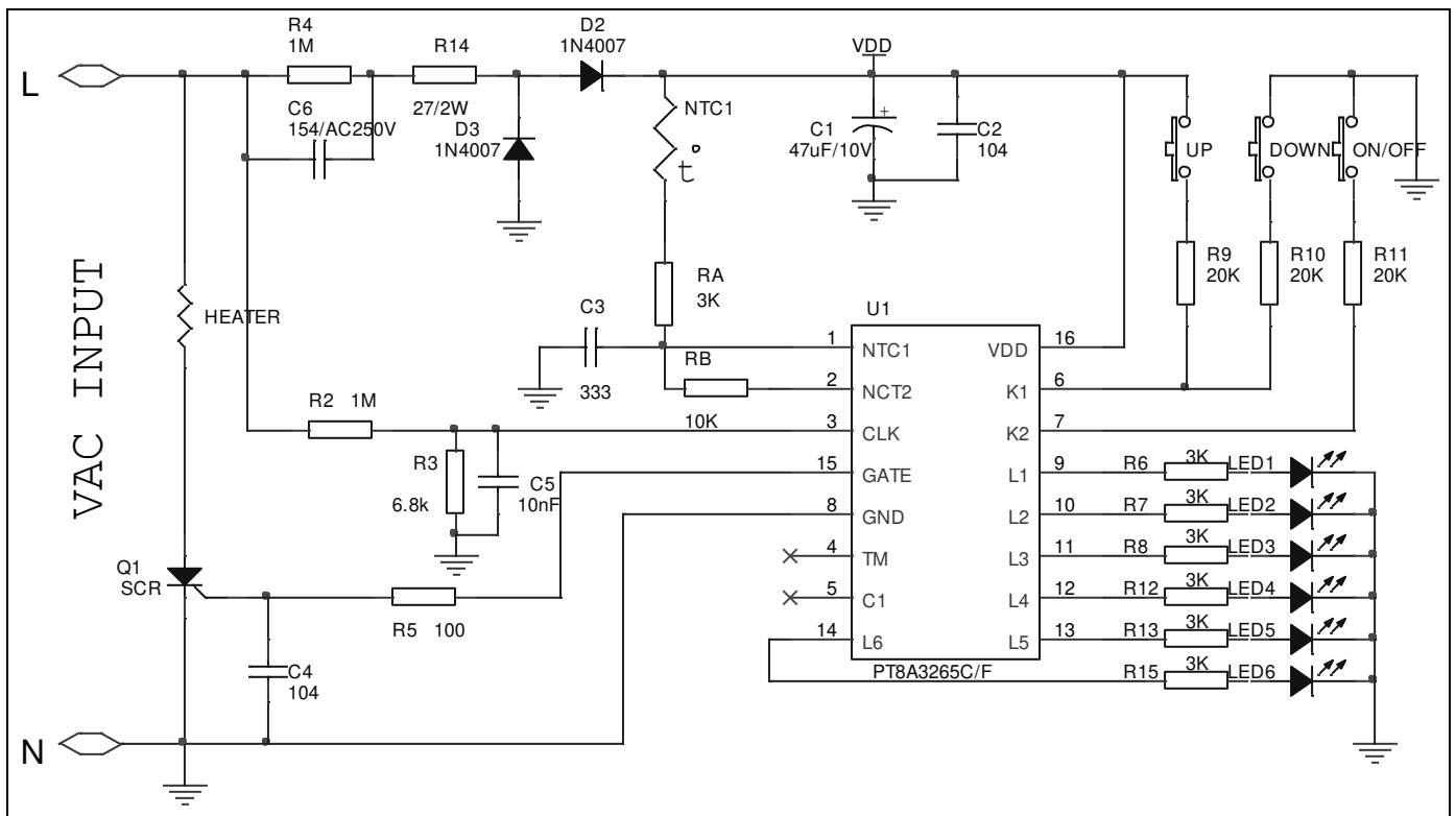
Application circuit for PT8A3265C/F
