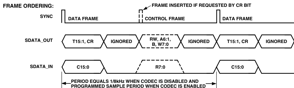
Figure 10. Frame Ordering
